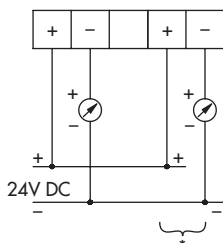
Fig. 5-2: Electrical connection
