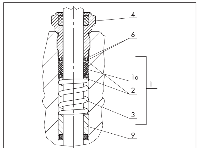
Fig. 9: PSA packing · DN 15 to 50/NPS ½ to 2
