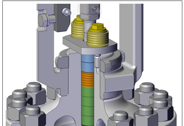
Fig. 4: Live-loaded packing with packing flange (loaded by external springs) with tightening option
