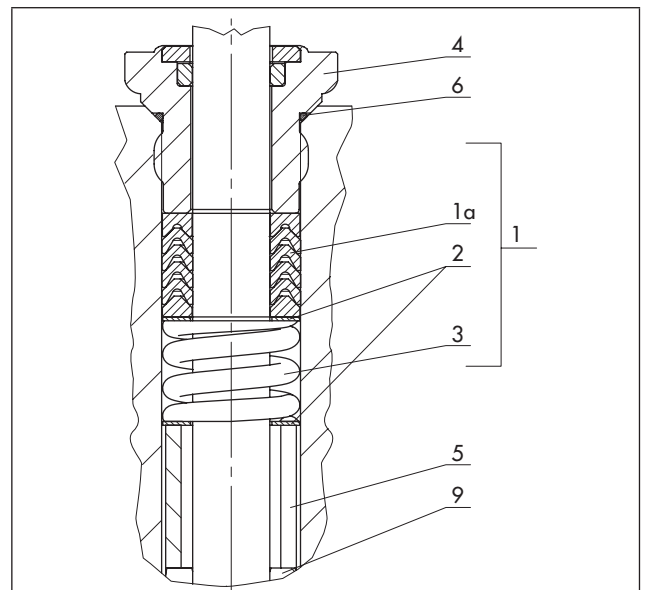
Fig. 10: Form LT packing · DN 65 to 80/NPS 2½ to 3
