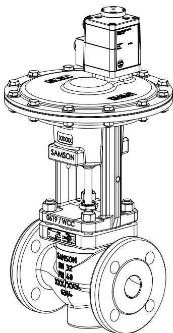
Fig. 2: Type 3351 with directly attached solenoid valve
