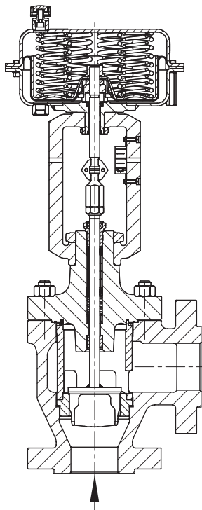
Fig. 2: Type 3296-1 Control Valve with Type 3271 Actuator
