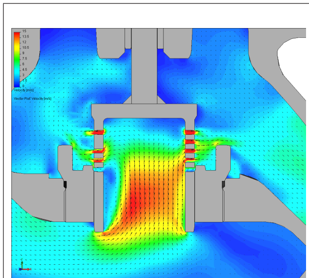
Fig. 3: Type 3251 Globe Valve, flow-to-open
