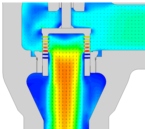
Fig. 4: Type 3256 Angle Valve, flow-to-close
